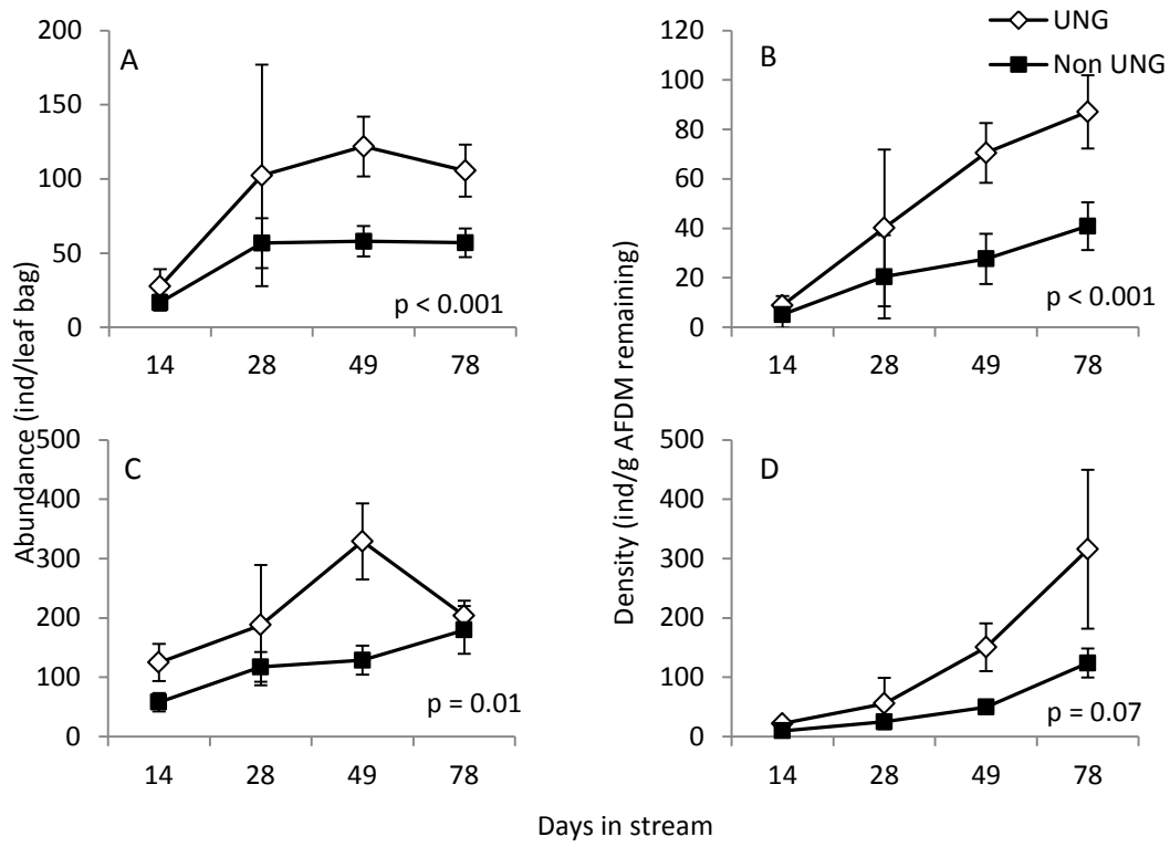
Figure 8. Fall deployment mean ( \pm 1 SE) FM macroinvertebrate abundance (A) and density (B) and CM macroinvertebrate abundance (C) and density (D) over time in streams with and without UNG. Error bars on some dates are too small to be seen. AFDM = ash-free dry mass. P-values from paired t-test of total means.
