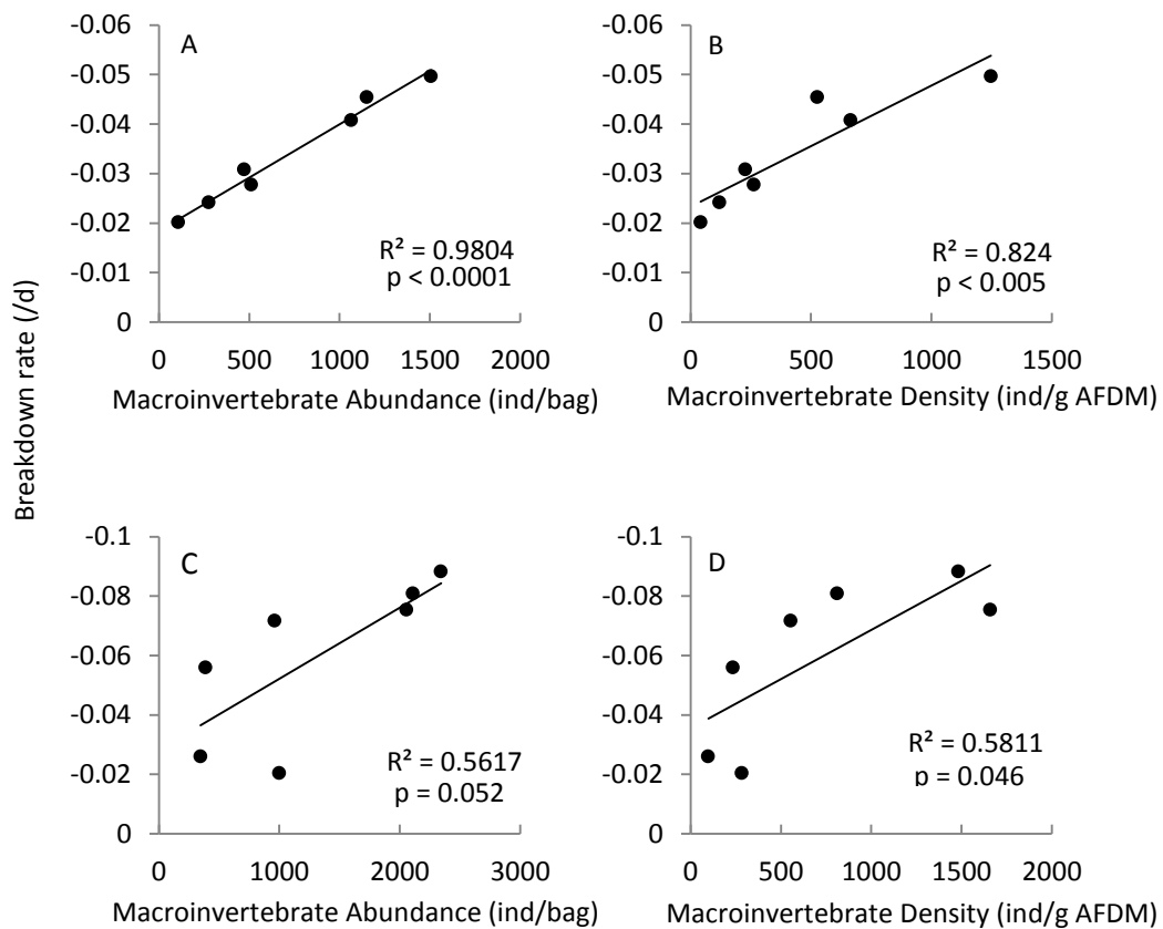
Figure 6. Linear regression of summer deployment leaf breakdown rates and FM macroinvertebrate abundance (A) and density (B) and CM macroinvertebrate abundance (C) and density (D). AFDM = ash-free dry mass. Note difference in x-axis scales between FM and CM regressions.
